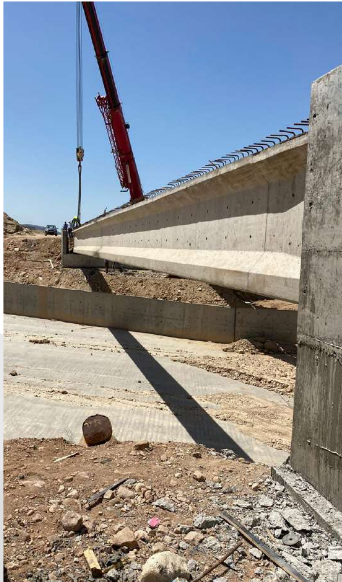
Protection Works For Bridges Along Dead Sea – Ghor Hadetha –Road –Package 2, 2021.
